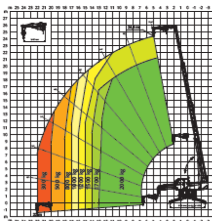
JIB WITH WINCH 2,000 kg
