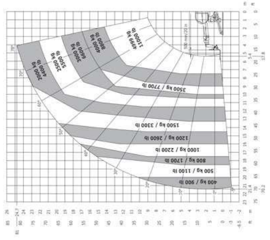
Rotation on lowered stabilizers with forks
